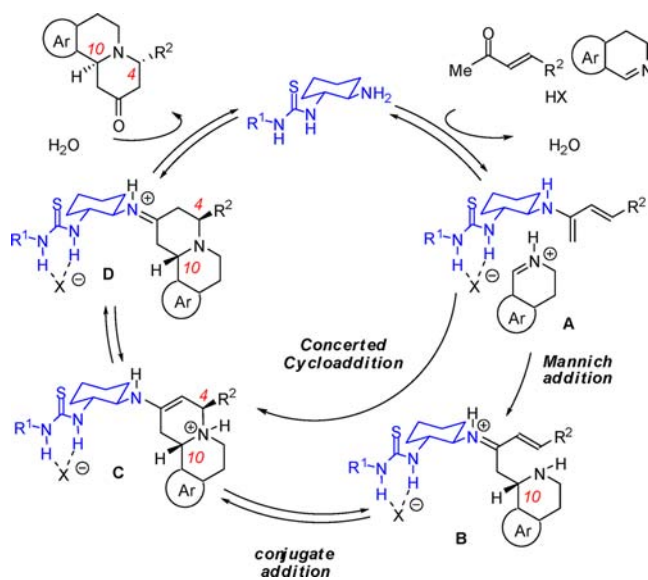
Scheme 3. Possible C4-Epimerization Pathways
