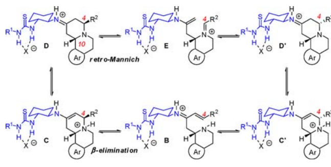
Scheme 3. Possible C4-Epimerization Pathways
